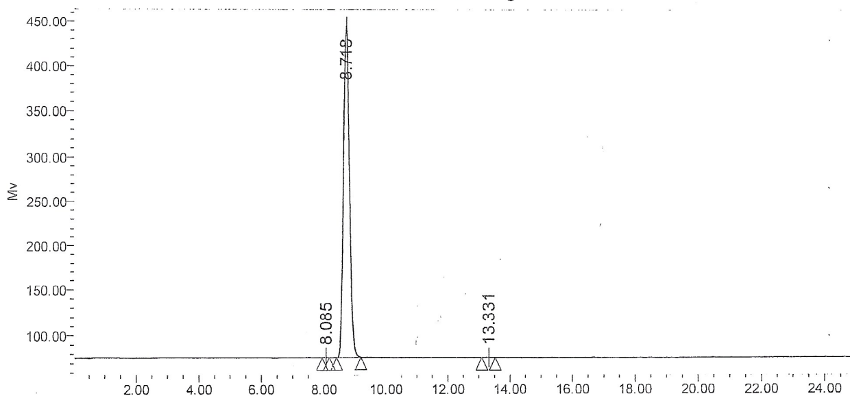
Auto-Scaled Chromatogram
